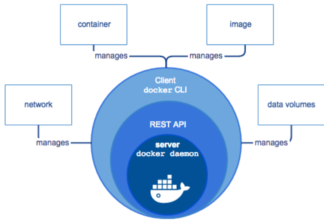
Figure 15: Docker Engine Architecture
